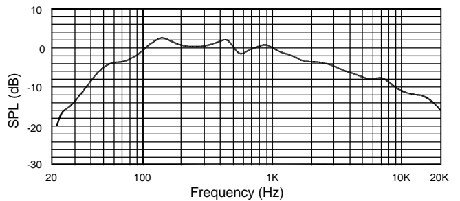
Normalized Response \pm 45^\circ VERTICAL 1/3 Oct. Avg.
