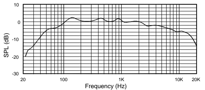
Normalized Response \pm 15^\circ VERTICAL 1/3 Oct. Avg.
