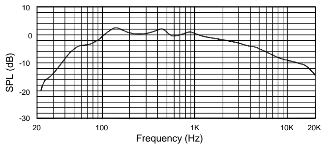
Normalized Response \pm 30^\circ VERTICAL 1/3 Oct. Avg.
