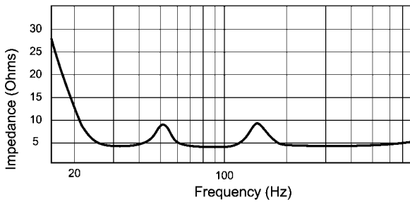
ARSO-215 Impedance
